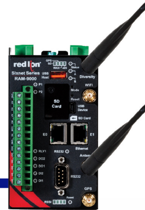
RAM® 9000 Cellular RTU with I/O
